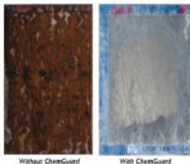
ASTM B117 Salt Spray 1000 Hours of Exposure
